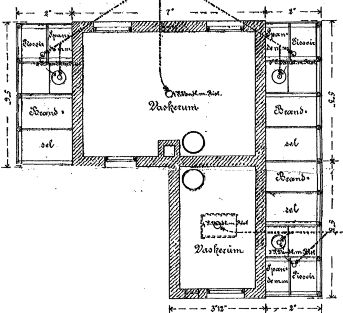
Plan of Type IV. 1 Skk.
