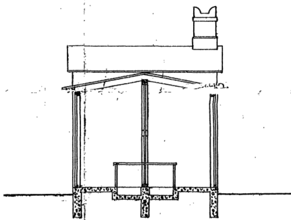
Snit E-F.
